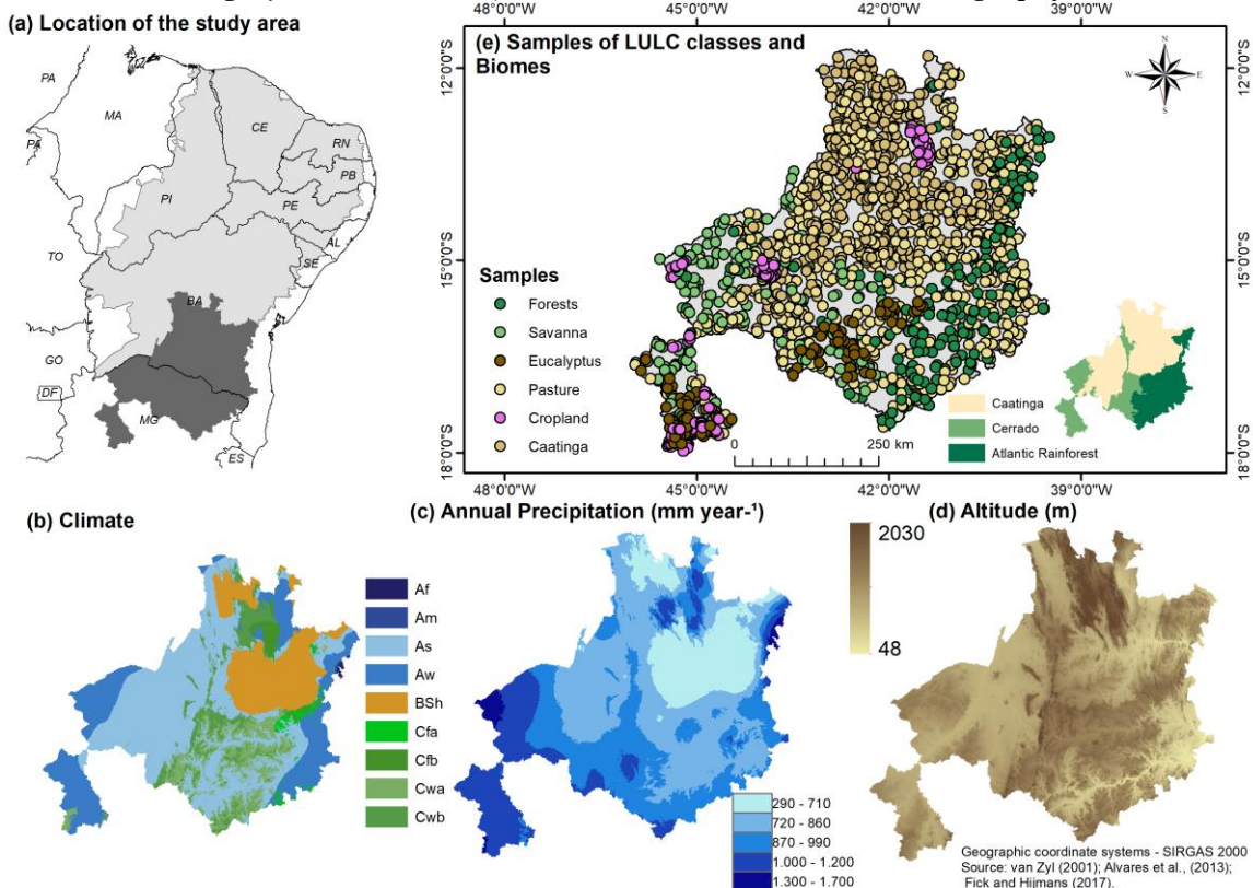
Figure 1 – Location map of the study area: (a) Brazilian semi-arid region (light gray) and the area considered in the present study (dark gray); (b) different climate types according to Köppen's classification; (c) distribution of annual precipitation (1970 – 2000); (d) altimetric variations; (e) LULC samples used, as well as the Brazilian biomes of the region according to the Instituto Brasileiro de Geografia e Estatística (IBGE – Brazilian Institute for Geography and Statistics)
