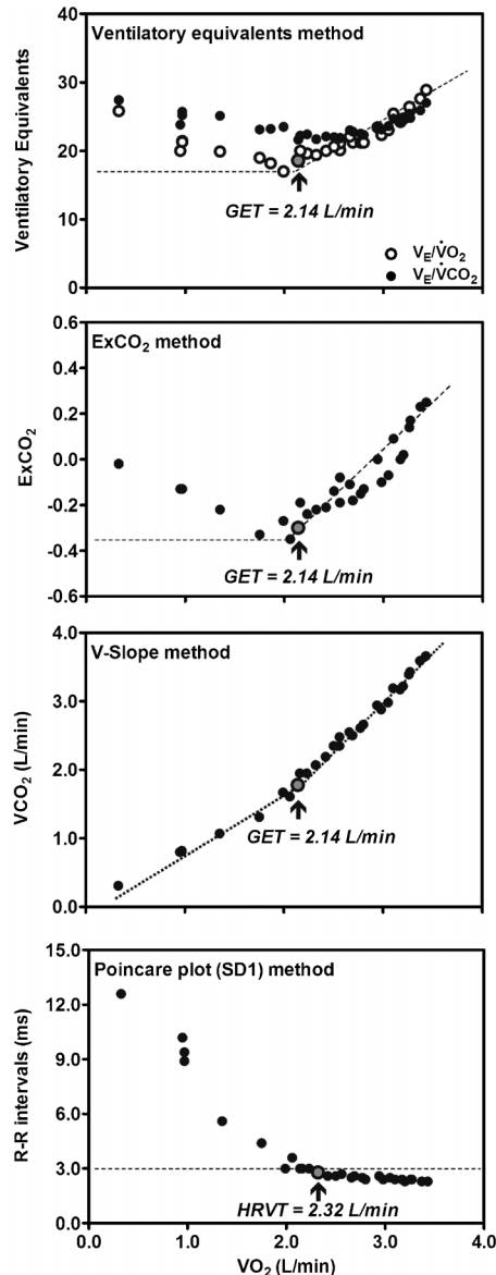
Figure 1. Graphic illustration of the methods used to determine the gas exchange threshold (GET; ventilatory equivalents method, excess \text{CO}_2 method, V-slope method) and heart rate variability threshold (HRVT; Poincare plot method).
