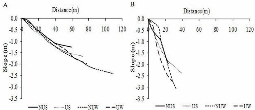
Fig. 2. Shore profiles of the Shangri-lá (A) and Barra do Sul (B) beaches: non-urbanized sector - summer (NUS), urbanized sector - summer (US), non-urbanized sector - winter (NUW), urbanized sector - winter (UW).
