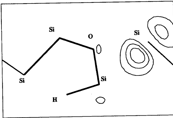
Figure 2. Electronic density for the empty gap state at the metastable configuration. Contours run from 0.02 to 0.10 electrons/ \text{\AA}^3 .
