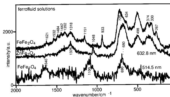
Figure 1. Raman spectra of Fe and Zn edl-ff in solution. The lower spectrum was excited at 514.5 nm.
