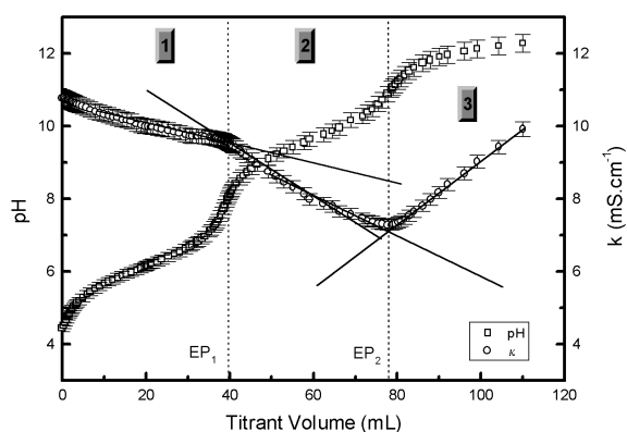
Figure 2. Simultaneous conductimetric-potentiometric titration curves of the dihydrate of the EDTA sodium salt titration. The regions 1 and 2 refer to the titration of H_2Y^{2-} and HY^{3-} species, respectively. The region 3 corresponds to the excess of base titrant. The equivalence points are determined by the technique of graphical directions lines.
