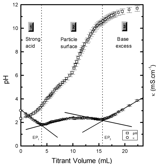
Figure 4. Simultaneous conductimetric-potentiometric titration curves of sample B. The regions indexed 1, 2 and 3 correspond to the strong acid titration (bulk solution), the weak acid \equiv MOH_2^+ and amphoteric \equiv MOH superficial sites titrations and the base excess respectively. EP_1 and EP_3 are determined by the technique of graphical directions lines.
