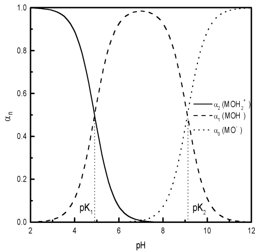
Figure 5. Speciation diagram of superficial sites for samples B. \alpha_n is the molar ratio of each superficial site, where n denotes the number of associated protons. For \text{pH}=7.0 , there is an isoelectric point.
