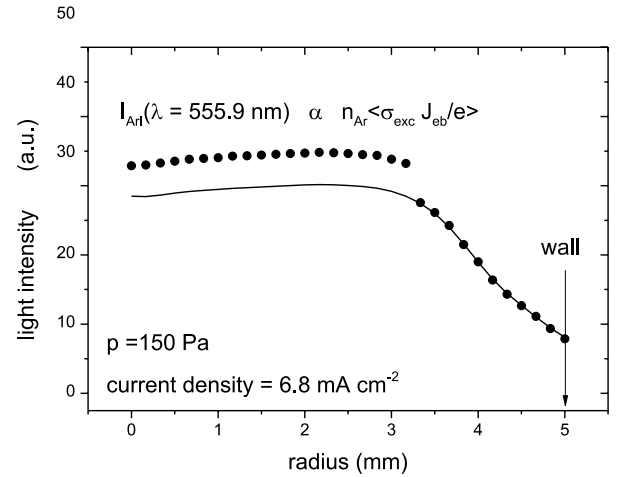
Figure 3. Radial profiles of the light intensity of the Ar I line at 555.9 nm ( n_{Ar} \langle \sigma_{exc} J_{eb}/e \rangle , excitation rate of the argon atoms by collisions with beam electrons).
