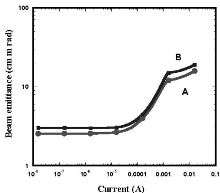
FIG. 9: Influence of current on beam emittance for spherical (A) and Pierce (B).
