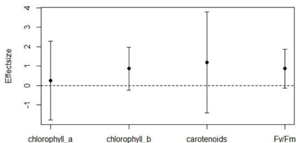
FIGURE 2 Effect size of toxic metals on chlorophyll a, chlorophyll b, carotenoids and Fv/Fm of Fabaceae species..
