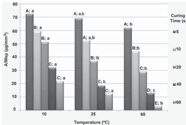
Figure 2- Comparison among values of composite sorption cured at different times and temperatures using the Mann-Whitney U test. Different letters indicate statistically significant differences when comparing both curing times at each temperature (uppercase letters) and temperatures at each curing time (lowercase letters) ( p < 0.05 )
