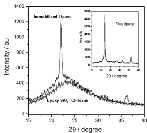
Figure 8. X-ray diffractograms for epoxy SiO 2 -chitosan and immobilized derivative. Inserted box shows diffractogram for free lipase.
