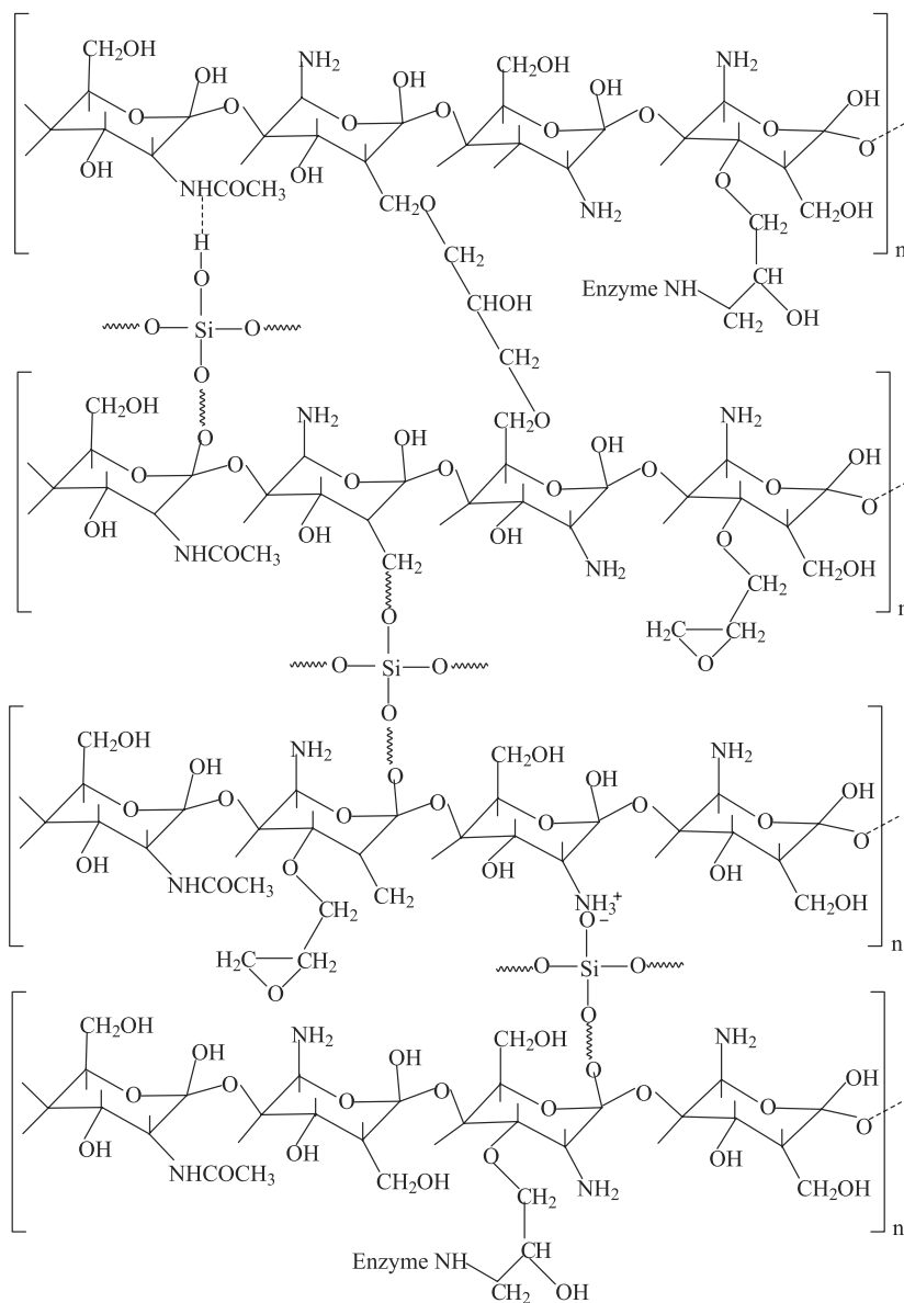
Figure 6. Proposed mechanism for SiO 2 -chitosan activation with epichlorohydrin and immobilization step.
