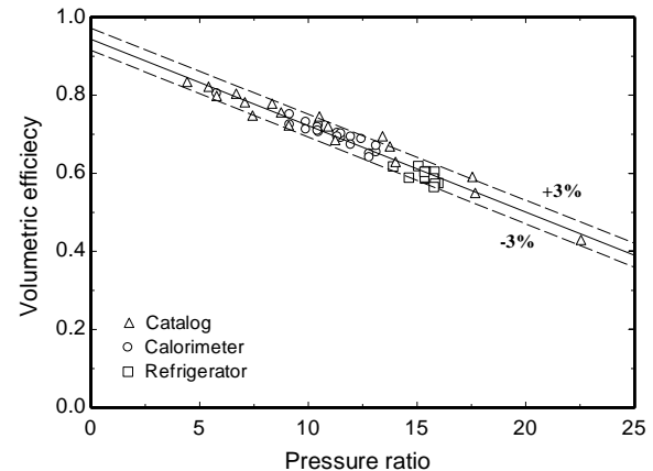
Figure 3. Correlation between the volumetric efficiency and pressure ratio.
