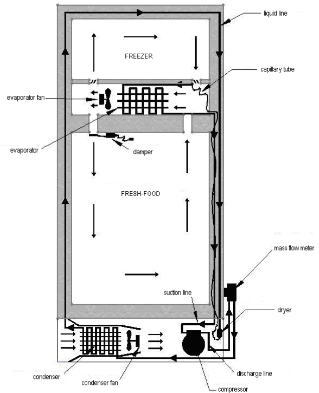
Figure 1. Schematic representation of the household refrigerator.
