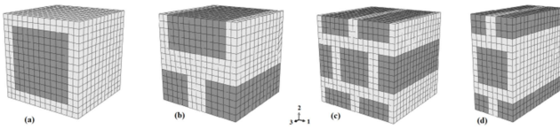
Figure 5. Finite Element Models for square section fiber: (a) square; (b) hexagonal; (c) hexagonal (shear 1-2) and (d) hexagonal (shear 2-3).
