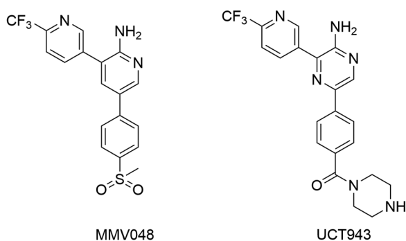
Fig. 17: PI4K inhibitors, aminopyridines compounds, MMV048 is in Phase 2 on clinical trials.
