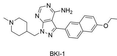
Fig. 12: bumped kinase inhibitor (BKI-1) able to Pf CDPK4 inhibit.
