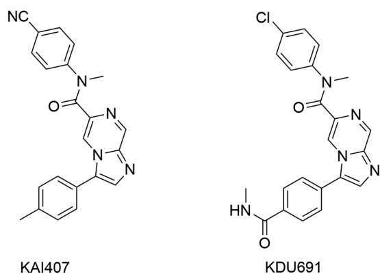
Fig. 16: imidazopyrazine compounds potential PI4K inhibitors.
