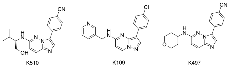
Fig. 13: inhibitors of Pf PKG, compounds K510, K109 and K497.
