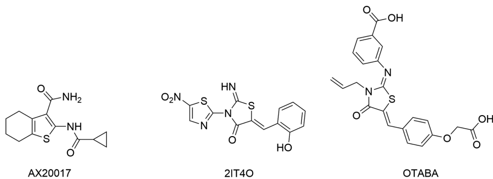
Fig. 10: kinase inhibitors active in Mycobacterium tuberculosis .
