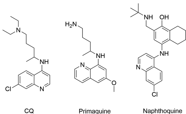
Fig. 4: chloroquine, primaquine and naphthoquine chemical structures.
