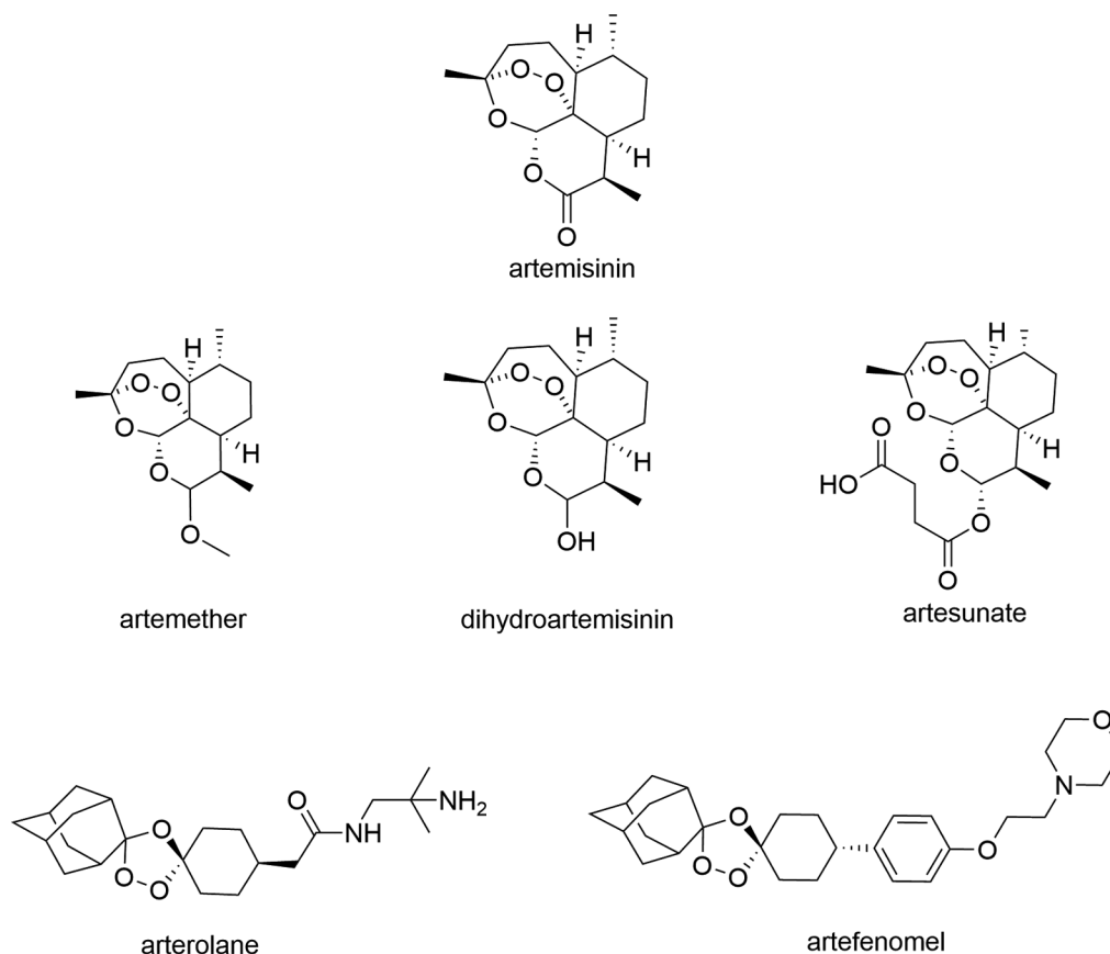
Fig. 3: artemisinin and its derivatives.
