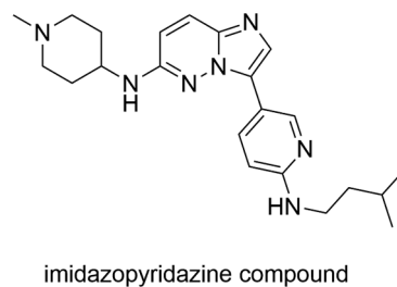
Fig. 11: imidazopyridazine derivatives, an inhibitor of Pf CDPK1.
