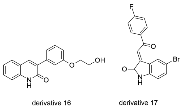
Fig. 15: quinolinone and oxindole derivatives, promising inhibitor of PfMRK .
