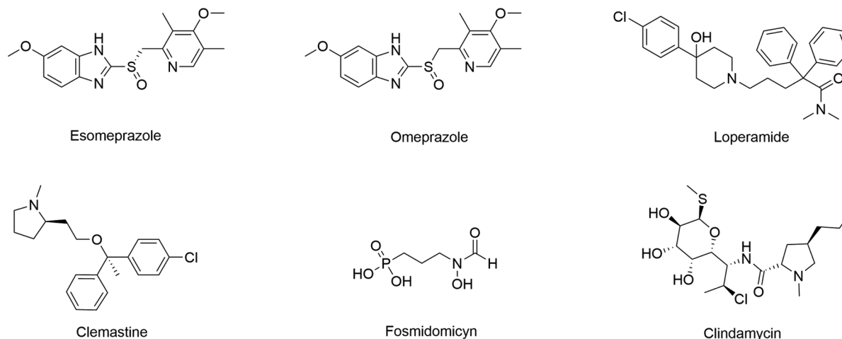
Fig. 7: repurposing drugs with activity on Plasmodium falciparum and P. berghei .
