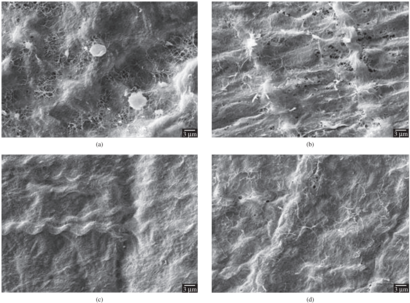
Figure 3. Scanning electron microscopy of bovine pericardium after crosslinking with glutaraldehyde (GA): a) 0.5% GA for 10 days; b) 0.5% GA for 10 days + glutamic acid/borate buffer; c) Pretreatment with GA 0.05% + 0.5% GA for 10 days; and d) Pre-treatment with GA 0.05% + 0.5% GA for 10 days + glutamic acid/borate buffer.
