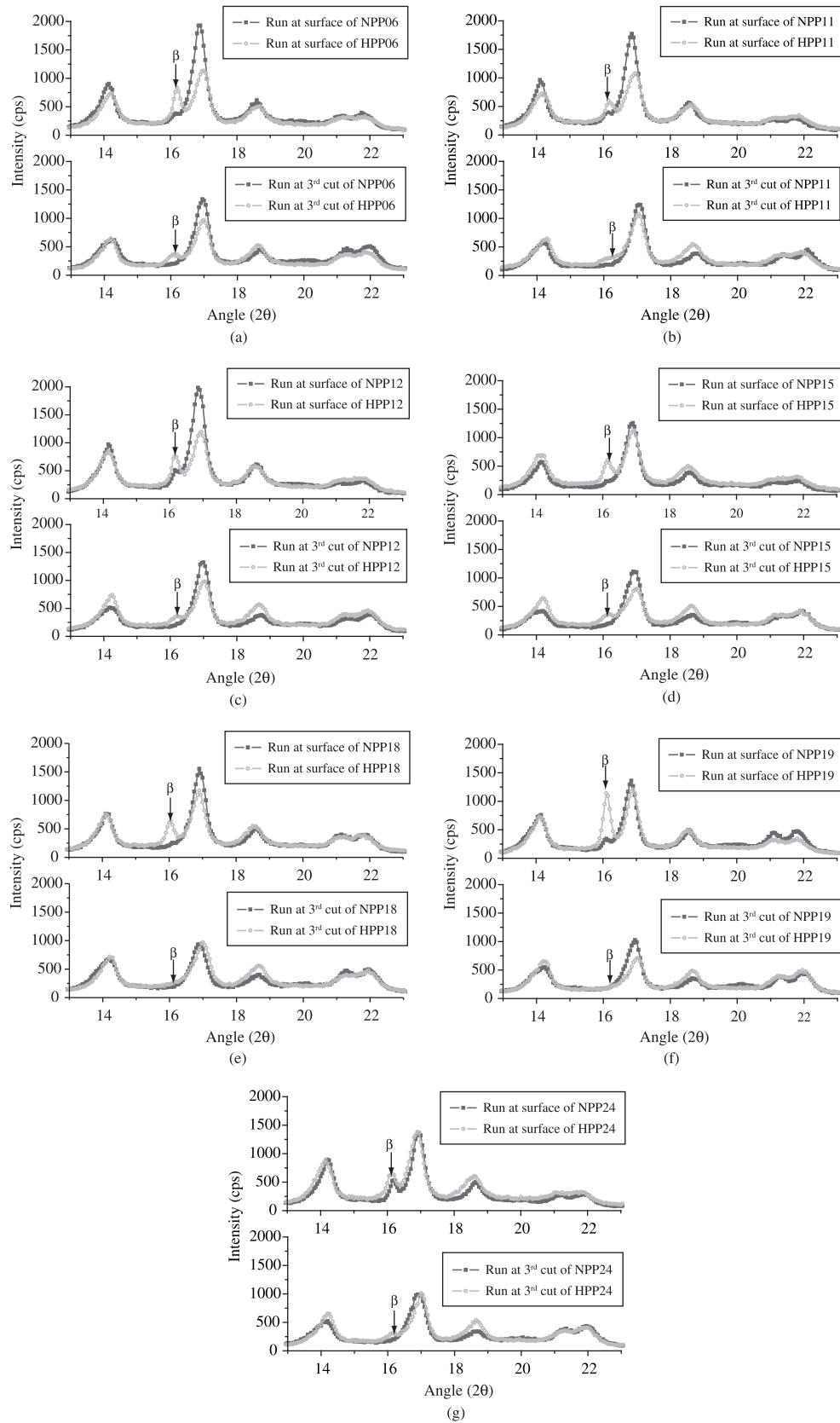
Figure 4. Diffractograms along the thickness of samples a) HPP06 and NPP06; b) HPP11 and NPP11; c) HPP12 and NPP12; d) HPP15 and NPP15; e) HPP18 and NPP18; f) HPP19 and NPP19; and g) HPP24 and NPP24.
