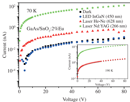
Figure 5. Current – voltage (I-V) curve for the heterojunction GaAs/ \text{SnO}_2 :2%Eu, in the dark and under illumination with distinct light sources, at 70 K. Inset: I-V curve for the same sample under the same conditions at 190 K. Data are plotted in log scale for better visualization of effects.
