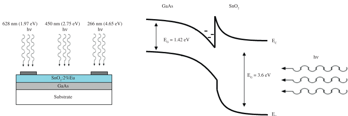
Figure 6. Schematic diagram of the sample structure, and the effects of monochromatic light irradiation on energy band diagram of GaAs/ \text{SnO}_2 :2%Eu sample.
