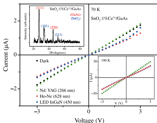
Figure 7. Current – voltage (I-V) curve for the heterojunction SnO 2 :1%Ce + /GaAs, in the dark and under illumination with distinct light sources, at 70 K. Inferior inset: I-V curve for the same sample under the same conditions, at 190 K. Superior inset: X-ray diffractogram for this heterojunction.
