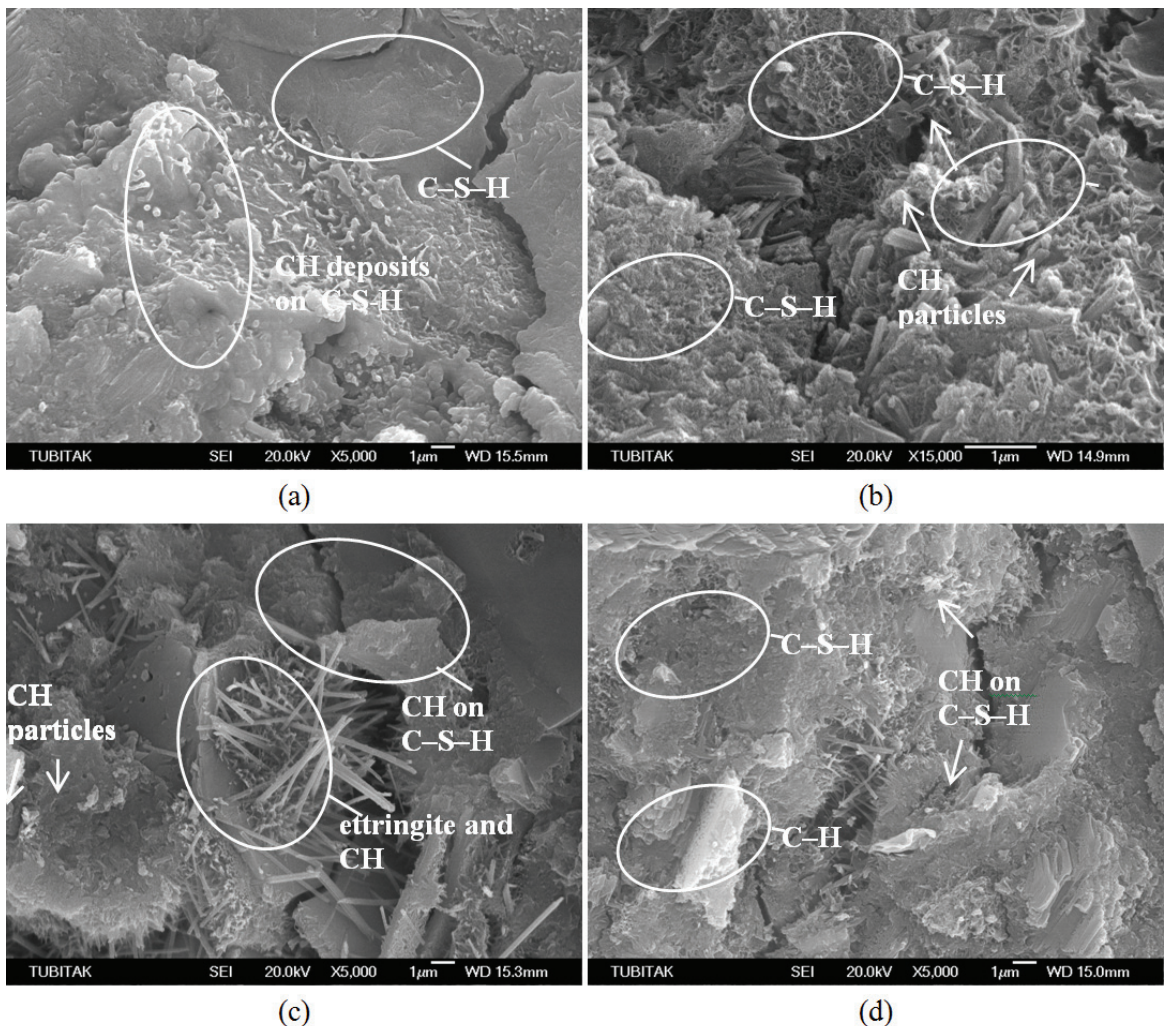
Figure 8. SEM images of the mortar specimens after 28 days of curing: a) OPC (control group), magnification x5,000; b) NS10, magnification x15,000; c) SF10, magnification x5,000; d) FA10, magnification x5,000.
