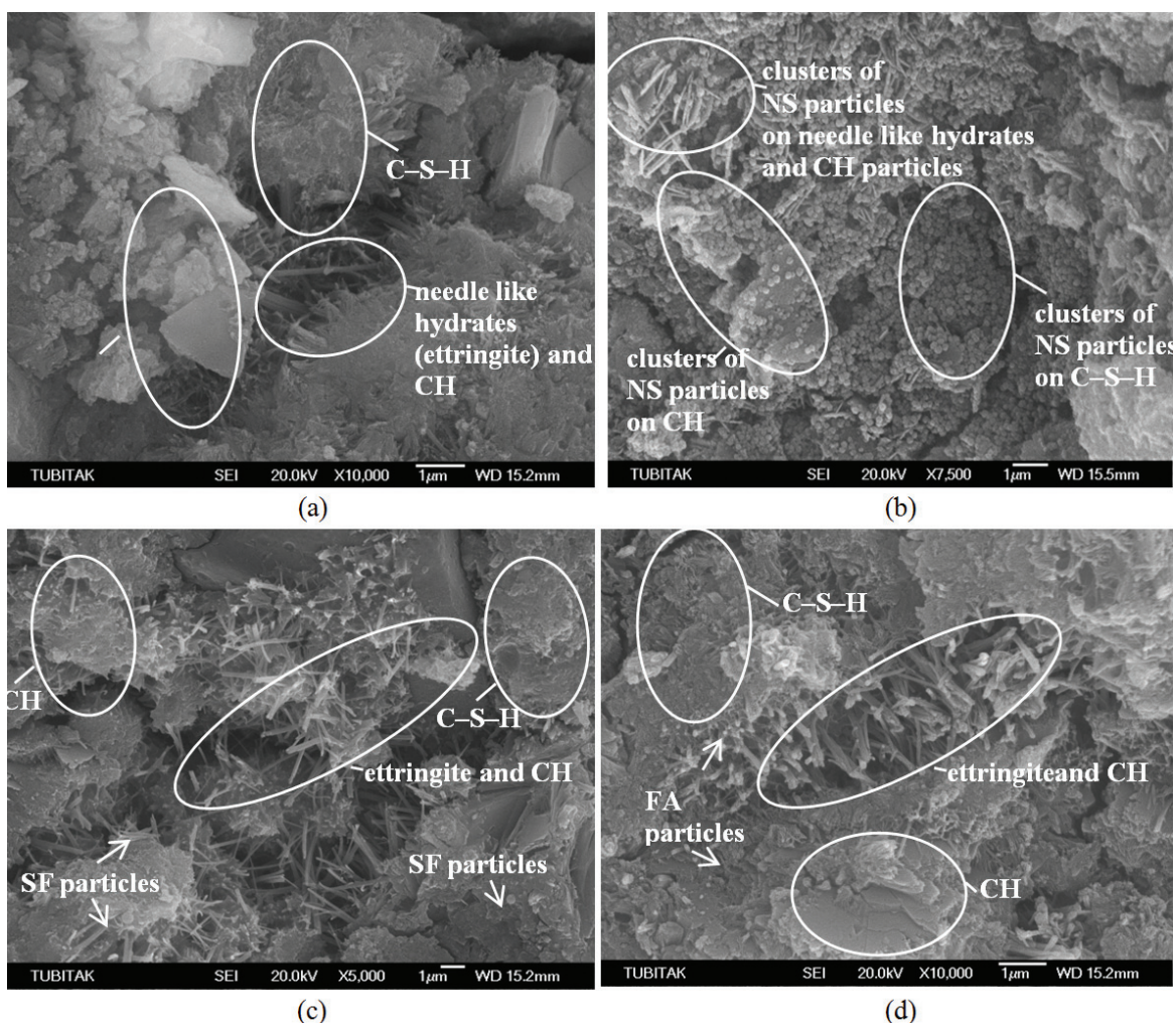
Figure 7. SEM images of the mortar specimens after 7 days of curing: a) OPC (control), magnification \times 10,000 ; b) NS10, magnification \times 7,500 ; c) SF10, magnification \times 5,000 ; d) FA10, magnification \times 10,000 .
