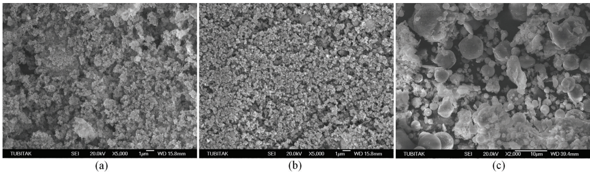
Figure 1. SEM images taken in this study for the pozzolanic additives: a) NS, magnification x5,000; b) SF, magnification x5,000; and c) FA, magnification x2,000.
