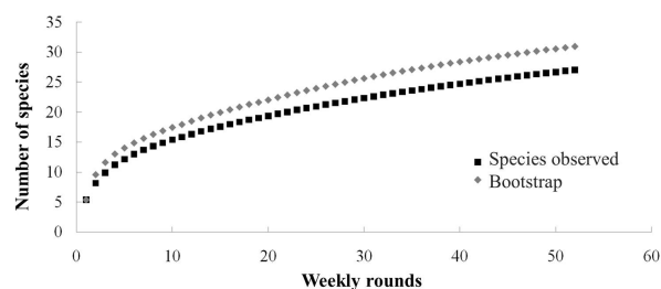
Figure 1 – Accumulation curve of species obtained with the Bootstrap estimator, through medium and large mammals records in 2012 in the Brasília National Forest Area 1, DF.
