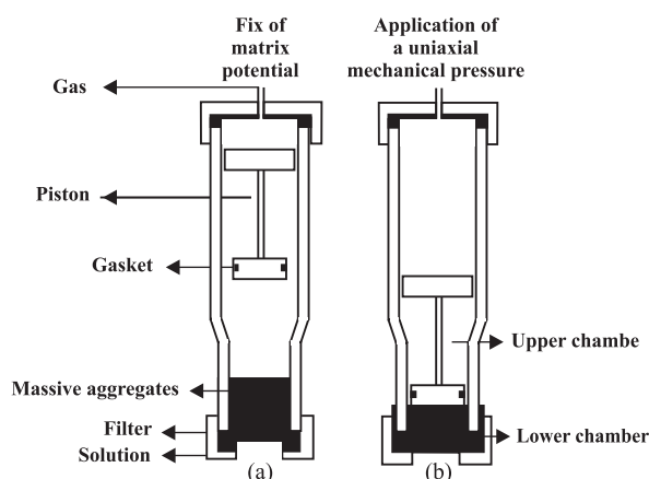
Figure 1. Mechanism used for this work: (a) fixation matrix potential (Tessier & Berrier, 1979) e (b) application of a uniaxial mechanical pressure (Sala & Tessier (1993), Apud Tavares Filho et al. (2005).
