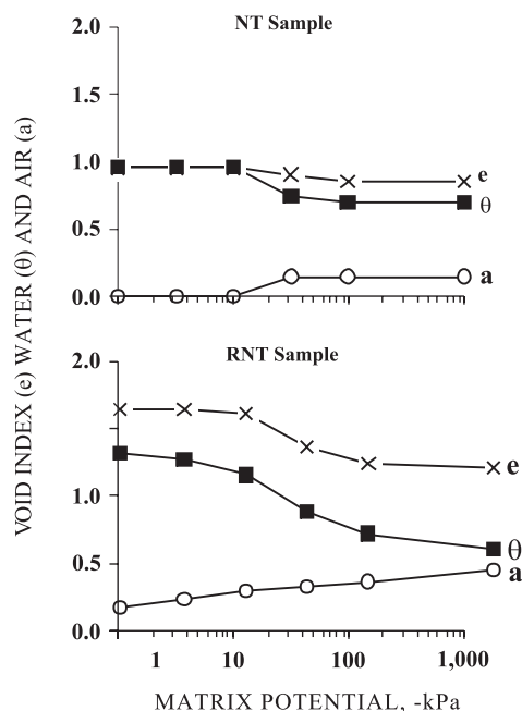
Figure 2. Index of voids (e), water ( \theta ) and air (a), average of five repetitions of clusters aggregates of 4 to 5 mm in diameter, of Oxisol under NT (no-till without crop rotation) and RNT (no till with crop rotation).
