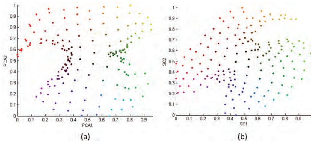
Figure 8 – SOM using a) a PCA projection and b) a Sammon projection. The hue is proportional to \tan^{-1} \left( \frac{y-1/2}{x-1/2} \right) while the saturation is proportional to [(x - 1/2)^2 + (y - 1/2)^2]^2 , such that they map to the 2D (PCA or SC) reference space.
