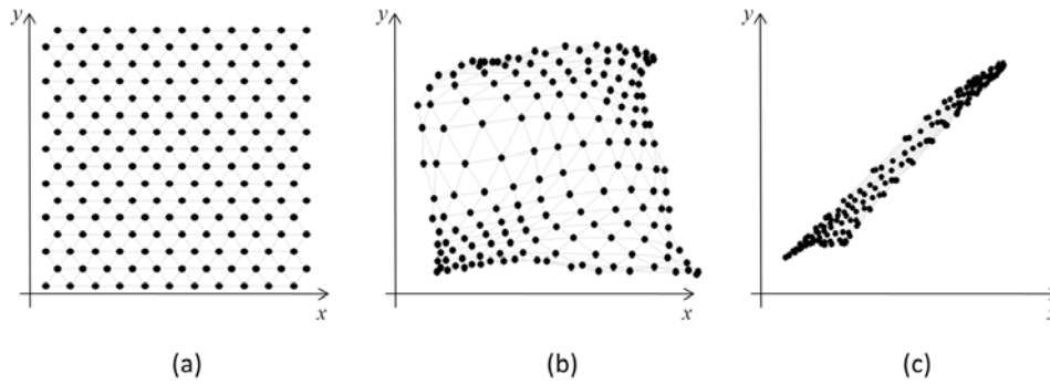
Figure 10 – Grid coordinates location during contraction. The (x, y) SOM grid coordinates are updated by Eq. (4).
