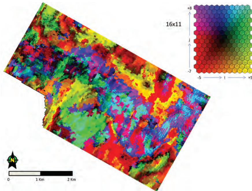
Figure 7 – 2D SOM with 16 \times 11 classes. Colors are a simple function of the prototype vector indices x_{ij} , where -5 \leq i \leq +5 and -8 < j \leq +8 . The hue is proportional to \tan^{-1}(j/i) while the saturation is proportional to (i^2 + j^2)^{1/2} .
