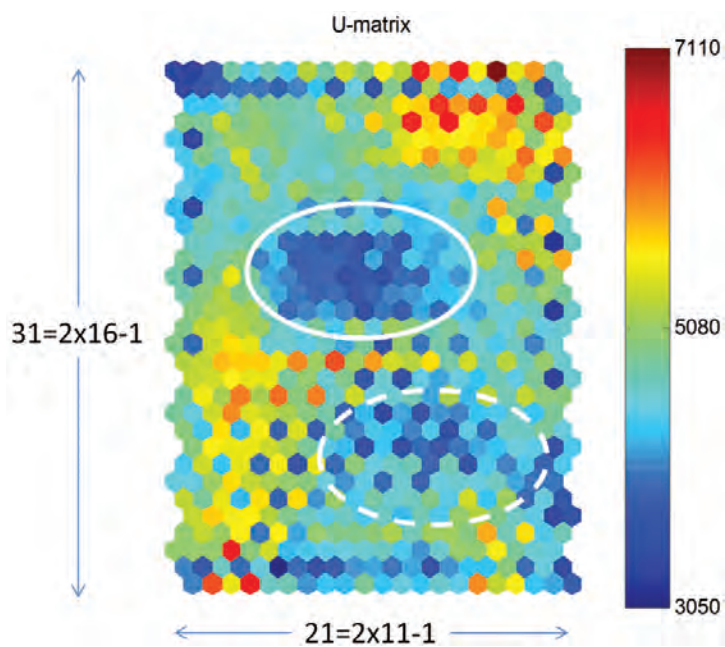
Figure 6 – U-matrix, where colors correspond to the distances between prototype vectors. U-matrix size is equal to twice 2D SOM size minus one (see Matos et al., 2007). Solid white ellipse indicates one good cluster. Dotted white ellipse indicates a more diffuse cluster. In general the data do not cluster well, but can still be ordered.
