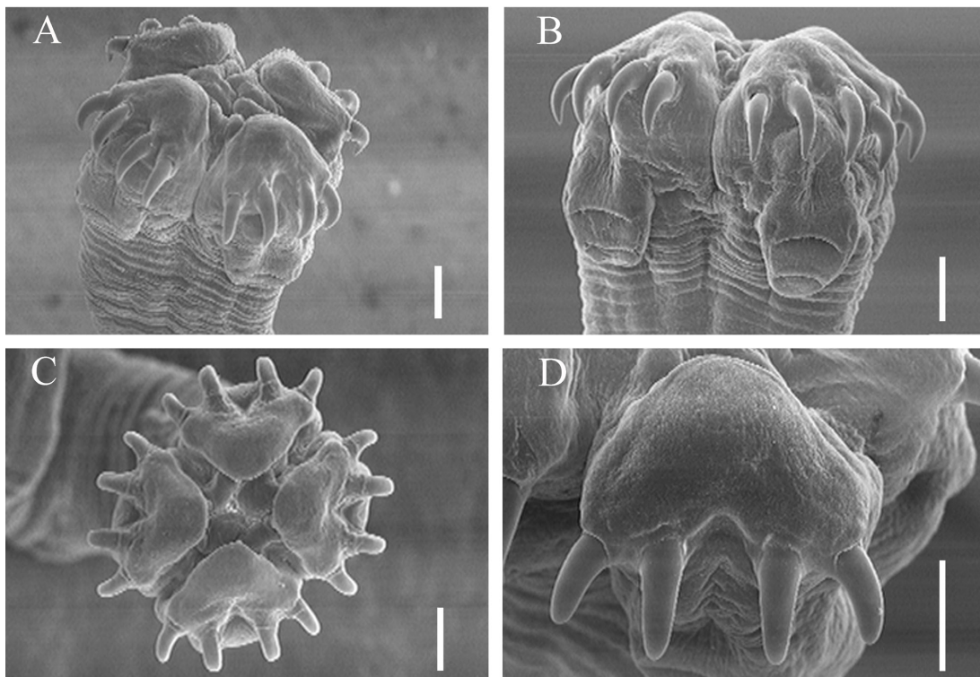
Figure 4. Scanning electron micrographs of Acanthobothrium marquesi n. sp. from Aetobatus cf. narinari . A. Scolex. B. Front view of pad, hooks and bothridia. C. Superficial apical view. D. Front view of pad and hooks. Scale bars: A, B, C, D 100 \mu m.
