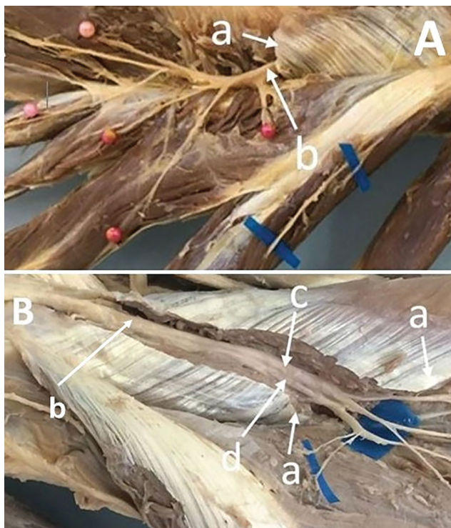
Fig. 8A Distal margins of the supinator muscle (a); Posterior interosseous nerve (PIN) (b) Distal branching to the distal margin of the supinator muscle. 8B - Distal margin of the supinator muscle (a); PIN (b); Superficial branch of the PIN (c) Deep branch of the PIN (d).
