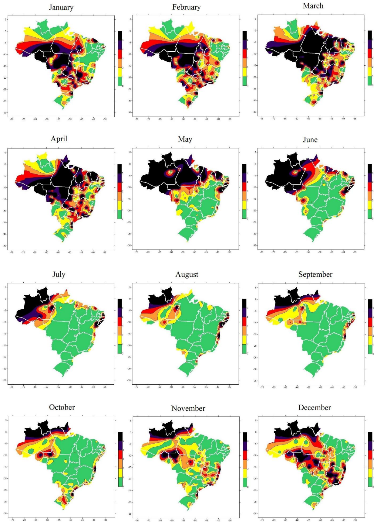
Figure 4. Risk zone maps for P. kuehni infection in Brazil from January to December 2008 developed based on the average of daily favorable hours (DFH) with temperatures between 17 and 24°C and humidity above 97%. 0 to 1 hours of favorability (green) = very low; 1 to 2 (yellow) = low; 2 to 3 (orange) = moderate; 3 to 4 (red) = high; 4 to 5 (blue) = very high and over 5 (black) = extremely high favorability.
