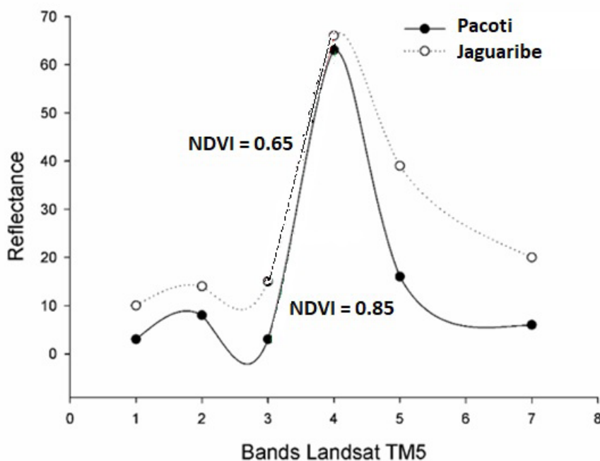
Figure 2. Reflectance and NDVI values obtained from the images of the Landsat TM5 from the two mangrove areas evaluated.
