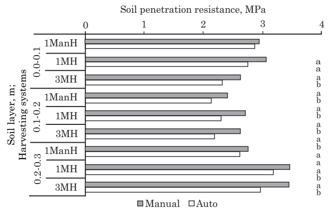
Figure 5. Comparison of mean values of soil penetration resistance (PR) obtained by penetrometer rod insertion by hand (Manual) and automated (Auto) in experimental sugarcane fields on a Rhodic Eutrudox, on which one manual harvest (1ManH), one mechanized harvest (1MH) and three mechanized harvests (3MH) were performed. Using the paired t test, bars followed by the same letters do not differ significantly ( p < 0.05 ) between introduction modes of the penetrometer rod in the same experimental area and soil layer.
