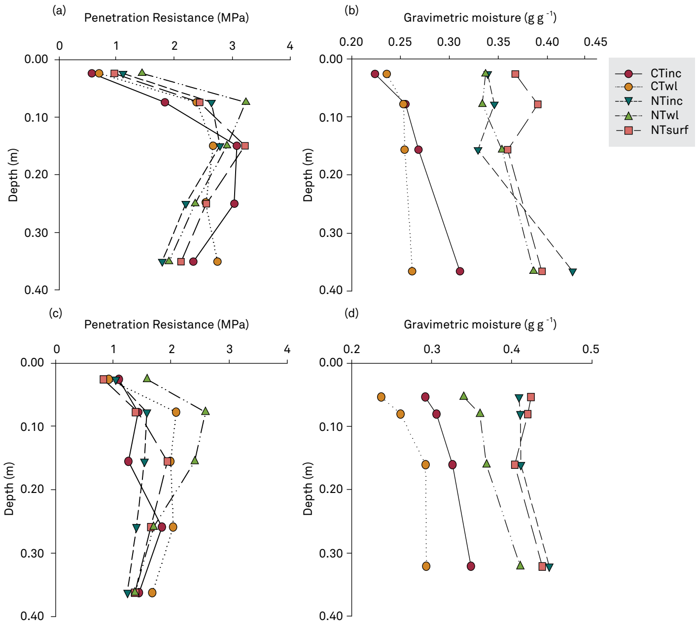
Figure 6. Penetration resistance (a, c) and gravimetric soil moisture (b, d) as affected by the tillage system and liming methods, in May 2009 (a, b) and March 2011 (c, d) in a Latosolo Bruno Alumínico típico (Hapludox). CTinc: conventional tillage with incorporated lime; CTwl: conventional tillage without lime; NTinc: no-tillage with incorporated lime; NTwl: no-tillage without lime; and NTsurf: no-tillage with surface lime.
