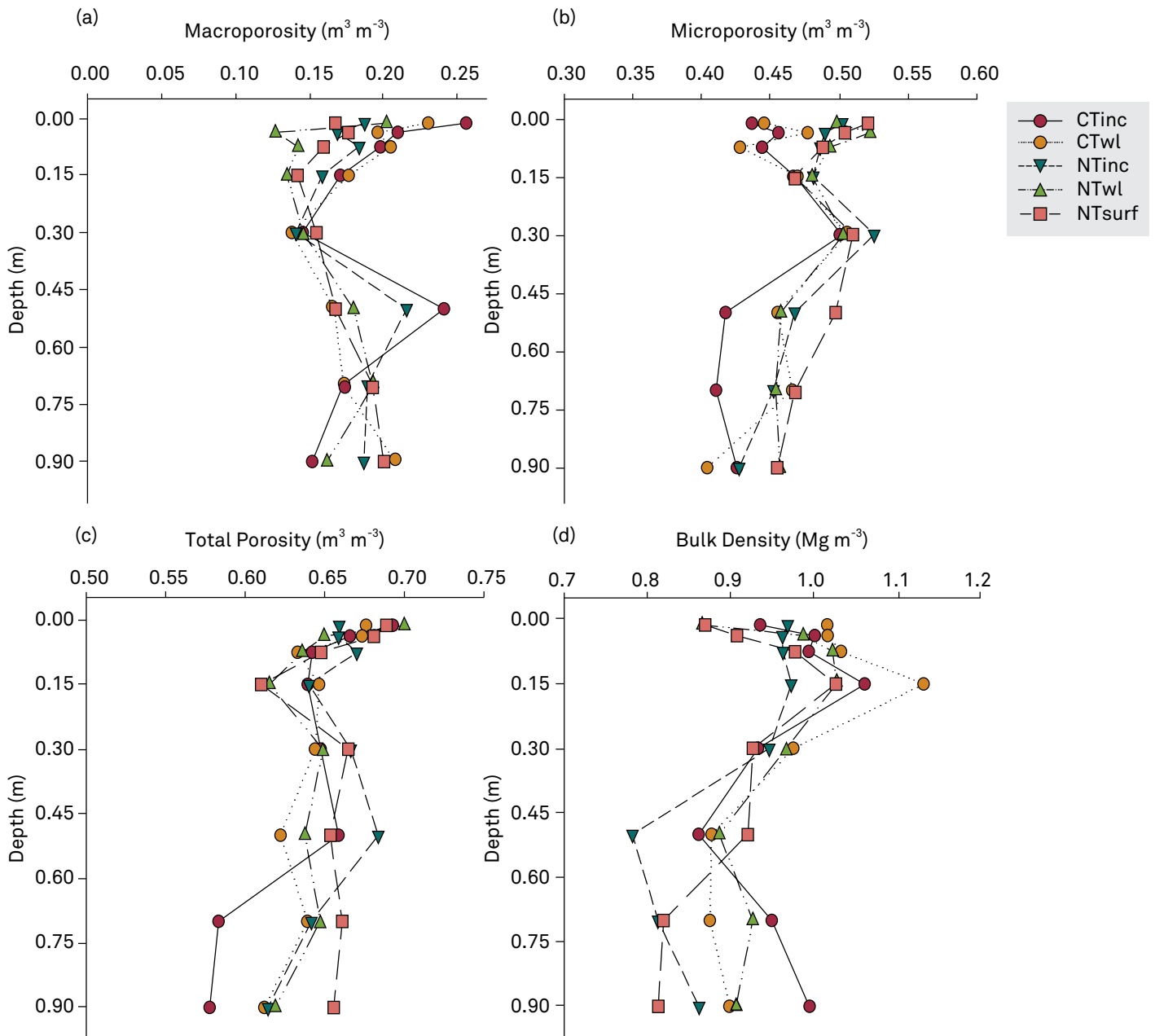
Figure 2. Macroporosity (a), microporosity (b), total porosity (c), and bulk density (d) in a Latossolo Bruno Alumínico típico (Hapludox) subjected to different tillage systems and liming methods. CTinc: conventional tillage with incorporated lime; CTwl: conventional tillage without lime; NTinc: no-tillage with incorporated lime; NTwl: no-tillage without lime; and NTsurf: no-tillage with surface lime.
