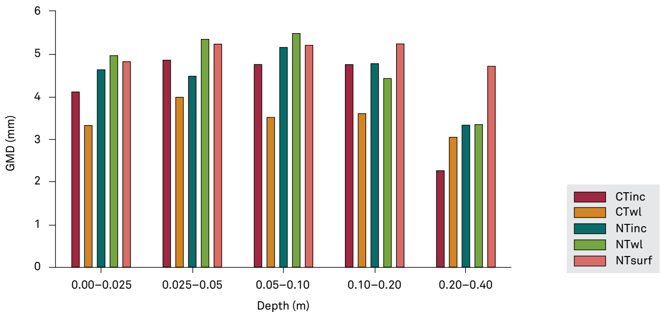
Figure 4. Geometric mean diameter (GMD) of soil aggregates as affected by tillage systems and liming methods at different depths of a Latossolo Bruno Alumínico típico (Hapludox). CTinc: conventional tillage with incorporated lime; CTwl: conventional tillage without lime; NTinc: no-tillage with incorporated lime; NTwl: no-tillage without lime; and NTsurf: no-tillage with surface lime.
