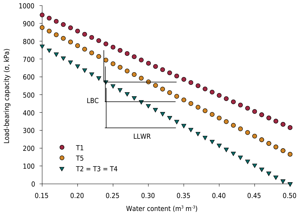
Figure 4. Variation in the load-bearing capacity (LBC) with water content ( \theta ) for a critical soil bulk density (BD) value of 1.57 \text{ Mg m}^{-3} in a Latossolo Vermelho Distroférico (Rhodic Hapludox) at the depth of 0.15 m, in T1, T5, and T2 = T3 = T4. T1 - single-shank ripper with chiseling at the depth of 0.15 m; T2 - single-shank ripper with chiseling at the depth of 0.30 m; T3 - two-bar ripper with chiseling at the depth of 0.15 m; T4 - two-bar ripper with chiseling at the depth of 0.30 m; T5 - control without chiseling. LLWR: least limiting water range.
