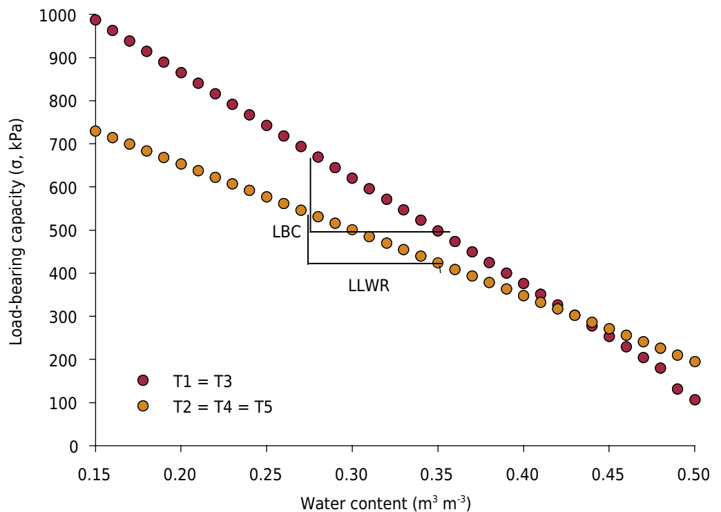
Figure 5. Variation in the load-bearing capacity (LBC) with water content ( \theta ) for a critical soil bulk density (BD) value of 1.55 \text{ Mg m}^{-3} in a Latossolo Vermelho Distroférico (Rhodic Hapludox) at the depth of 0.30 m, in T1 = T3 and T2 = T4 = T5. T1 - single-shank ripper with chiseling at the depth of 0.15 m; T2 - single-shank ripper with chiseling at the depth of 0.30 m; T3 - two-bar ripper with chiseling at the depth of 0.15 m; T4 - two-bar ripper with chiseling at the depth of 0.30 m; T5 - control without chiseling. LLWR: least limiting water range.
