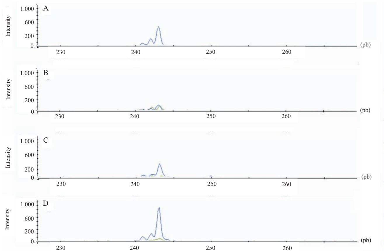
Figure 2. Peak intensity of different treatments are shown using polymerase chain reaction (PCR) purification. All peaks resulted from IAC-SSR293 labeled with 6-FAM. A: control with no purification; B, C and D: tests with 0.5 \mu L, 1 \mu L and 1.5 \mu L purified DNA, respectively. The highest intensity peak was found for 1.5 \mu L PCR-purified product (D).
