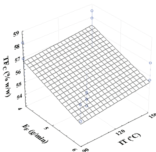
Figure 4. Surface response plot of total flavonoid content as a function of drying air inlet temperature and extract feed rate.
