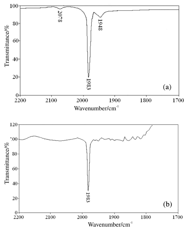
Figure 2. Spectra of [W(CO) 6 ] in hexane solution (a) after immediate contact with Pd sin t/ \gamma -Al 2 O 3 ; (b) after 6 h contact with Pd/ \gamma -Al 2 O 3 .
