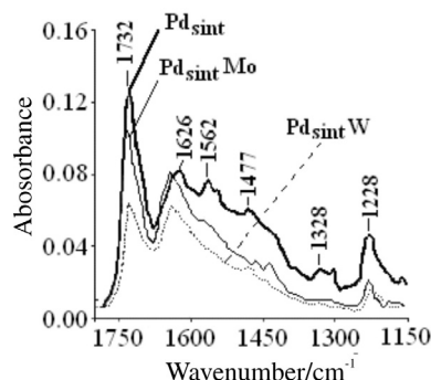
Figure 5. FTIR spectra of the \nu(\text{NO}) region of Pd sint / \gamma\text{-Al}_2\text{O}_3 , Pd sint -Mo/ \gamma\text{-Al}_2\text{O}_3 , Pd sint -W/ \gamma\text{-Al}_2\text{O}_3 catalysts after 5 min NO exposure followed by 2 min under vacuum.
