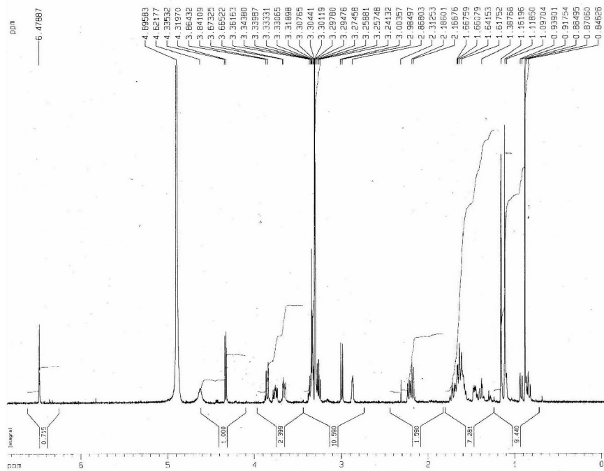
Figure S9. ^1\text{H} NMR spectrum of 2 (500MHz, \text{CD}_3\text{OD} ).
