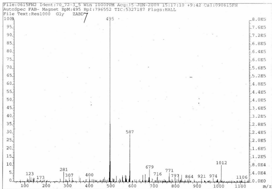
Figure S15. FABMS(-) spectrum of 2 ( \text{CD}_3\text{OD} ).
