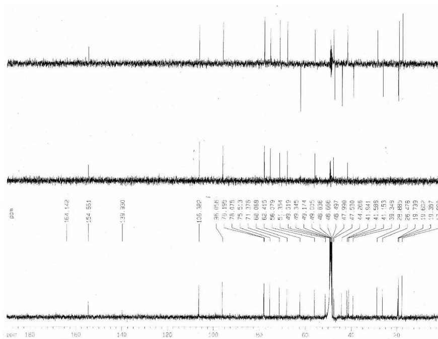
Figure S10. ^{13}\text{C} NMR (DEPT) spectrum of 2 (125MHz, \text{CD}_3\text{OD} ).
