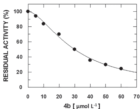
Figure 2. Inhibitory activity of compound 4b against rCPB2.8 enzyme.
