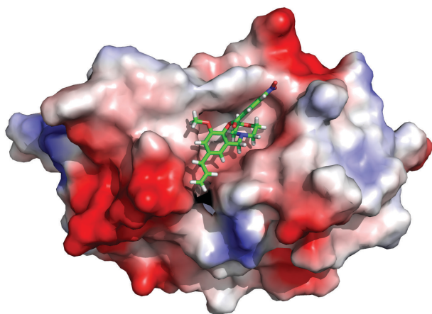
Figure 6. Electrostatic surface potential of the enzyme rCPB 2.8 bound to compound 4b (scale from -70.232 (negative, red) to 70.232 (positive, blue)).
