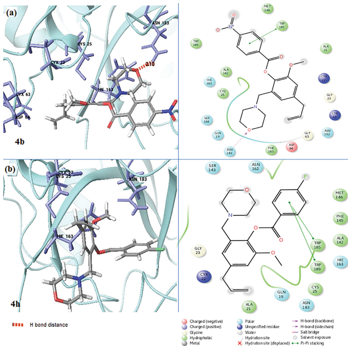
Figure 5. 3D structure representing the hydrogen bond between protein and ligand (orange dotted line), as well as the distance between the atoms that participate in this interaction, and 2D scheme demonstrating interactions between residues of the enzyme and the compounds (a) 4b and (b) 4h .
