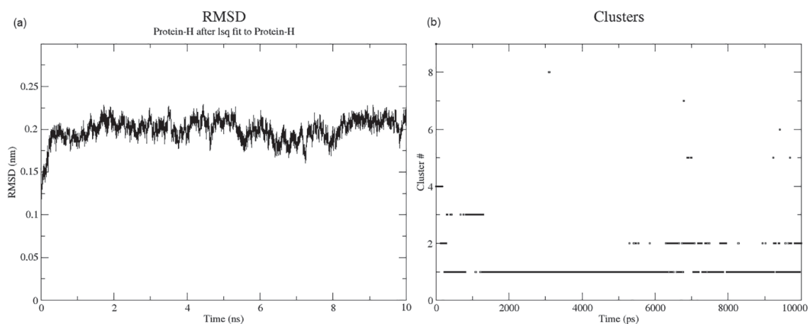
Figure 4. Simulation of molecular dynamics. (a) RMSD value calculated from the entire protein structure, except hydrogen atoms, obtained over time (ns); (b) cluster with approximate structures having low RMSD variation between them (cut-off value of 0.1 \text{ \AA} ) throughout the DM simulation.
