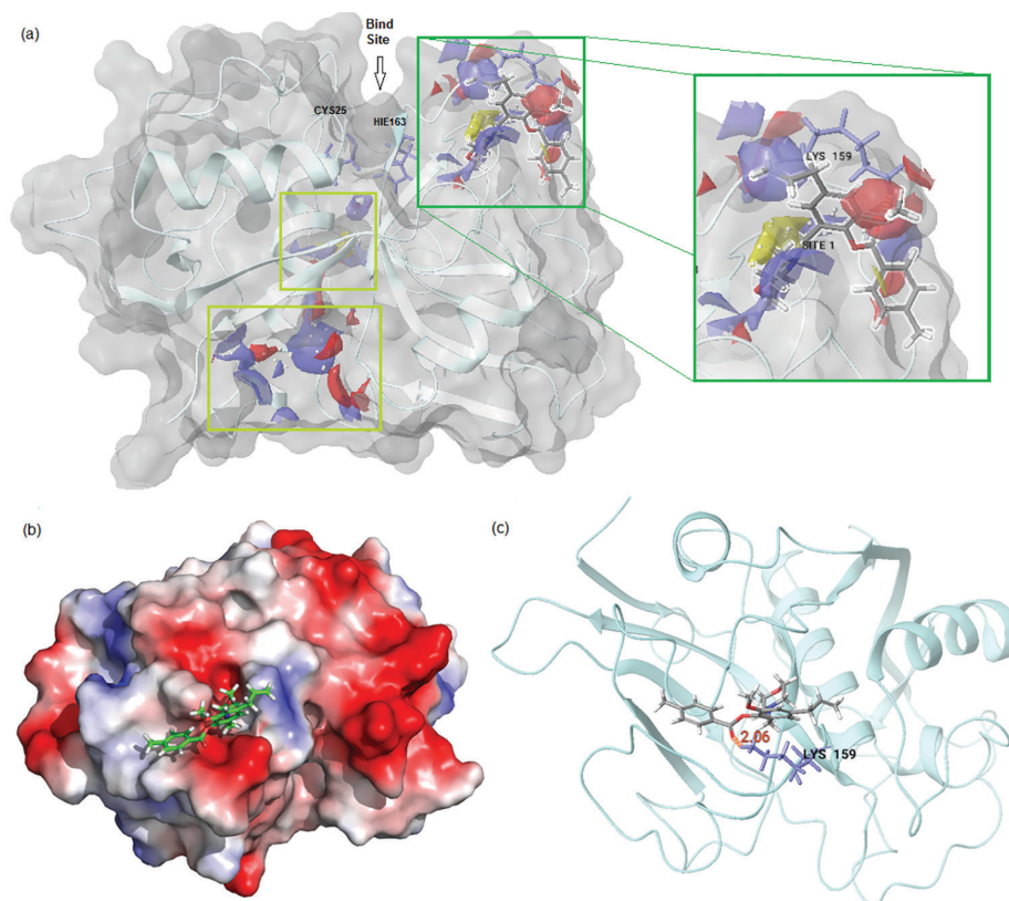
Figure 8. Interaction profile between compound 4c and the “interaction site 1” of rCPB 2.8. (a) The surface of the rCPB 2.8 enzyme with the active site and the 3 sites of interaction predicted by the SiteMap program (Schrödinger) highlighted in green, with the site with the best interaction profile linked to 4c compound; (b) electrostatic surface potential of the enzyme containing the ligand 4c at the allosteric site (scale -70.232 (negative, red) to 70.232 (positive, blue)); (c) ligand 4c forming a hydrogen bond with the residue LYS159 at the allosteric site.
