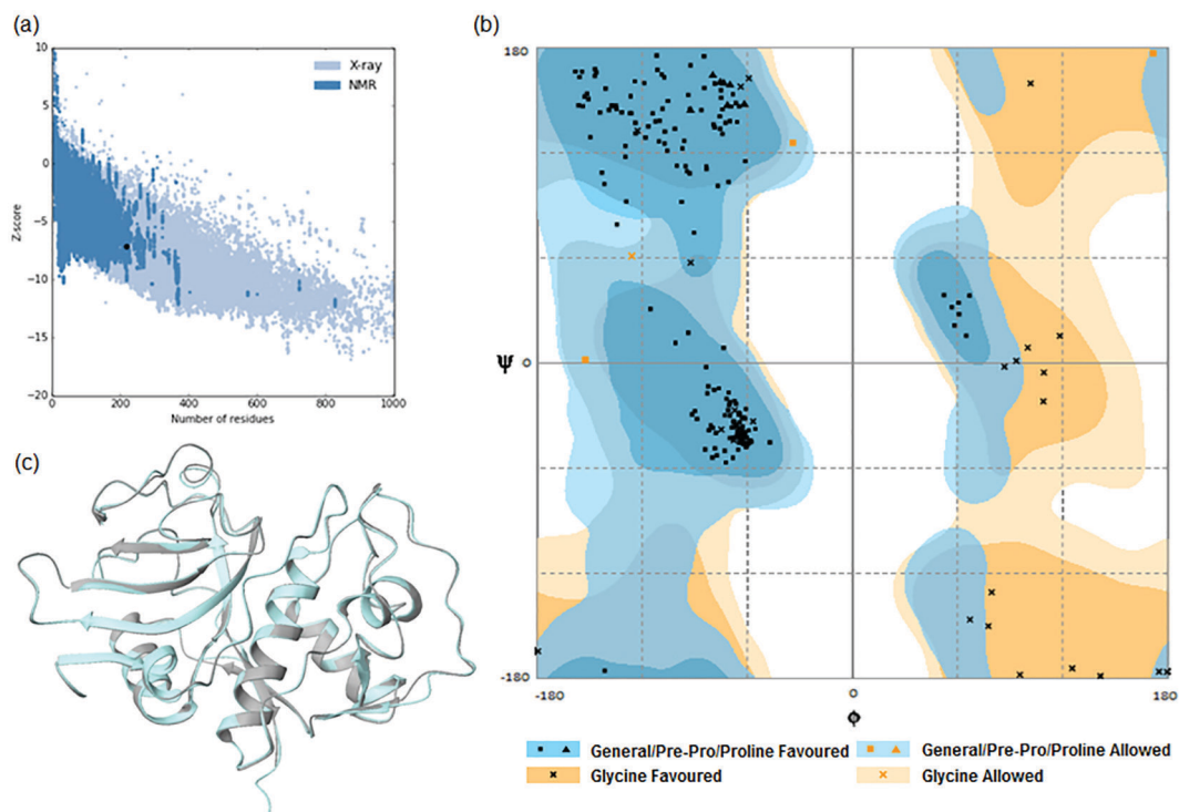
Figure 3. Model quality validation. (a) Z-score punctuation ( -7.11 ) of the model; (b) Ramachandran plot; (c) superposition of the homology model of rCPB 2.8 with the structure of cruzain used as template (PDB code: 3IUT).
