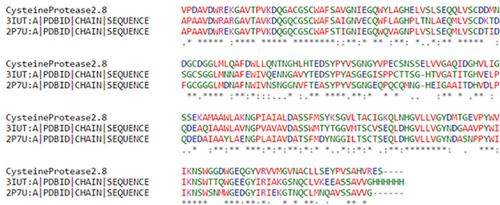
Figure 1. Multiple sequence alignment of rCPB 2.8 protein and templates (PDB code: 3IUT and 2P7U) performed by the Clustal Omega program. 24
