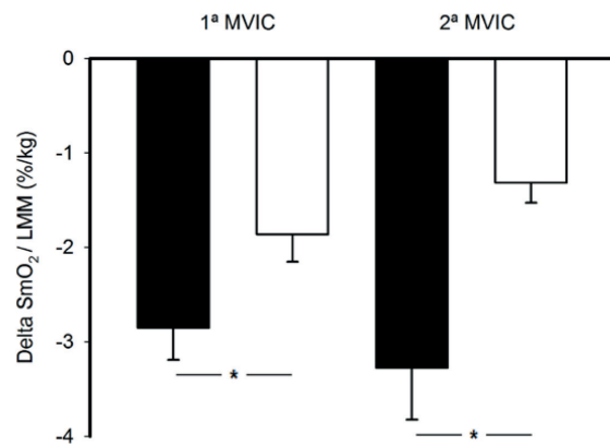
Figure 1 - Mean and Standard Deviation. O_2 muscle saturation delta adjusted by the leg muscle mass. Note the worst adaptation to stress in the COPD group by reducing muscle saturation. * P < 0.05 on the analysis between groups.
