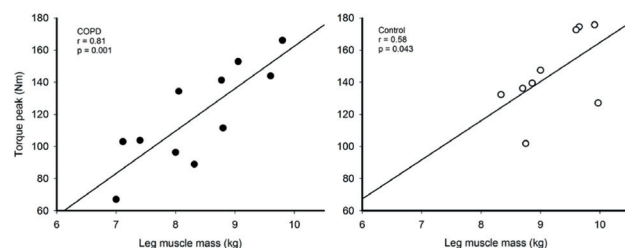
Figure 3 - Pearson's correlation. Nm - Newton meter. Note the significant influence of muscle mass in muscle strength, especially in the COPD group.
