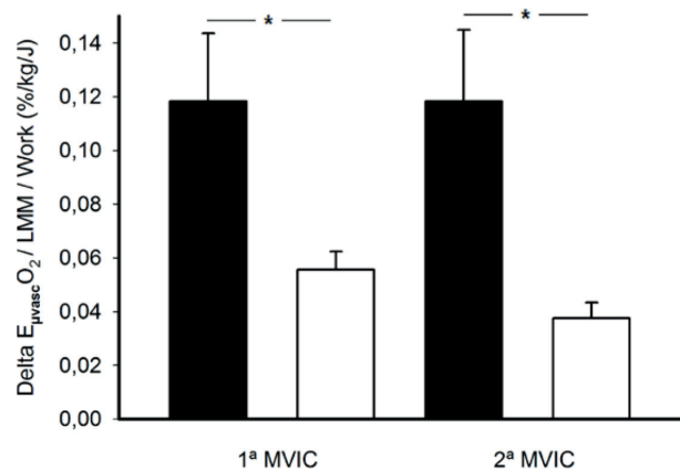
Figure 2 - Mean and standard deviation. Microvascular O_2 extraction delta corrected by the leg muscle mass (LMM) and the total work in the MVIC. Note the high energy cost according to the work performed by COPD group by mean of high O_2 extraction. * P < 0.05 on the analysis between groups.
