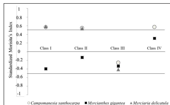
Figure 2 - Spatial distribution according to the Standardized Morisita's Index used in the population classes of three Myrtaceae species. Values that vary between -0.5 to 0.5 indicate a random distribution; values less than -0.5 indicate a uniform distribution; and values greater than 0.5 indicate an aggregated distribution.
