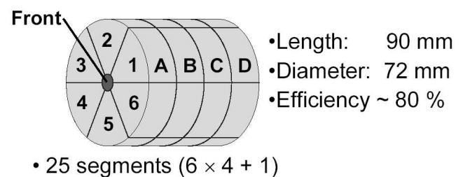
Figure 1. Schematic view of the 6 \times 4 + 1 segmented HPGe MARS prototype detector.
