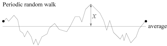
FIG. 6: A random walk on a finite interval with periodic boundary conditions. The random variable x represents the maximum deviation of the walk from its interval average. The probability distribution P(x) was calculated by Majumdar and Comtet [14].
