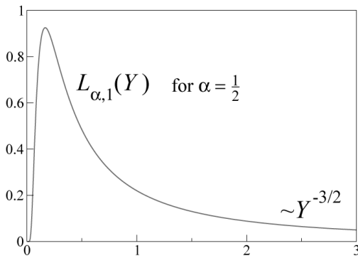
FIG. 1: The one-sided Lévy distribution L_{\frac{1}{2},1}(Y) is one possible outcome of a central limit theorem.
