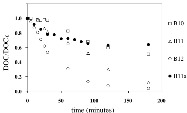
Figure 7: DOC/ \text{DOC}_0 -time curves for experiments with \text{DOC}_0 = 500 \text{ mg C L}^{-1} . B10 ( [\text{H}_2\text{O}_2] = 100 \text{ mmol L}^{-1} ; [\text{Fe(II)}] = 0.2 \text{ mmol L}^{-1} ); B11 ( [\text{H}_2\text{O}_2] = 188 \text{ mmol L}^{-1} ; [\text{Fe(II)}] = 0.4 \text{ mmol L}^{-1} ); B12 ( [\text{H}_2\text{O}_2] = 270 \text{ mmol L}^{-1} ; [\text{Fe(II)}] = 1.0 \text{ mmol L}^{-1} ); B11a ( [\text{H}_2\text{O}_2] = 188 \text{ mmol L}^{-1} ; [\text{Fe(II)}] = 0.4 \text{ mmol L}^{-1} ).
