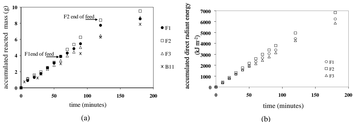
Figure 9: (a) Time evolution of the accumulated mass of carbon removed for the experiments B11, F1, F2, and F3 ( [H_2O_2] = 188 \text{ mmol L}^{-1} ; [Fe(II)] = 0.4 \text{ mmol L}^{-1} ). B11 (batch); F1 (fed-batch, 12 \text{ L h}^{-1} ); F2 (fed-batch, 6 \text{ L h}^{-1} ); F3 (fed-batch, 4 \text{ L h}^{-1} ). (b) Accumulated direct solar radiant energy in the fed-batch experiments.
