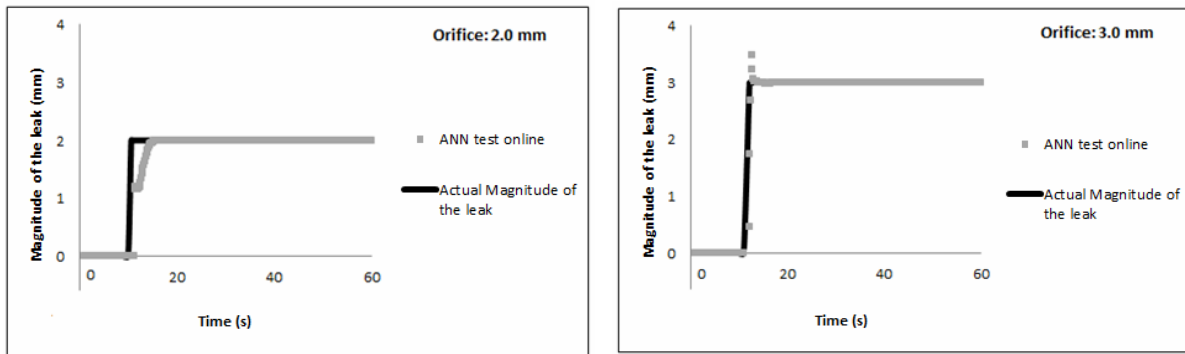
(a) Orifice diameter: 2.0 mm
