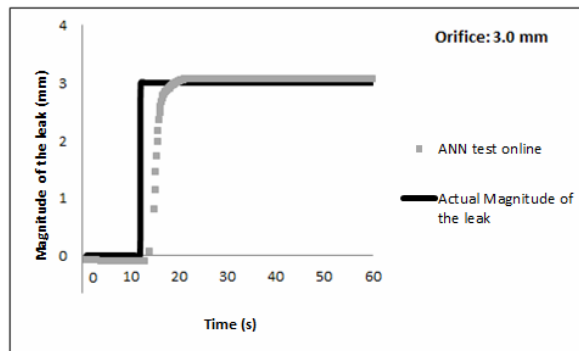
(c) Orifice diameter: 3.0 mm
