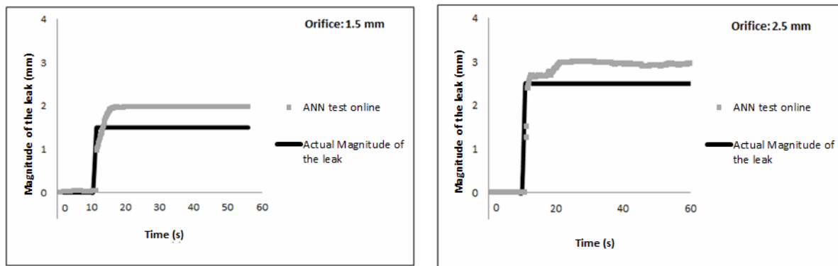
(a) Orifice diameter: 1.5 mm
