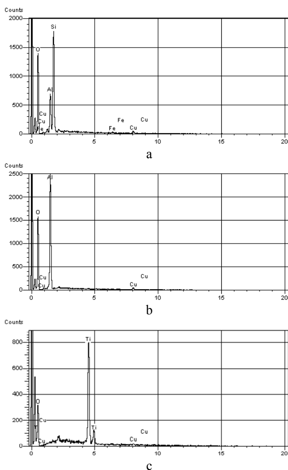
Figure 2: The EDX patterns of (a) CuO-PILC, (b) CuO/γ-Al 2 O 3 and (c) CuO-TiO 2 .
