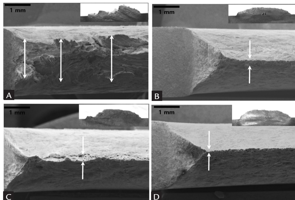
Figure 5 Fracture micrographs and profiles of the broken DENT ( l_0=17\text{mm} ). A) Alloy A 1050°C. B) Alloy B 1050°C. C) Alloy A 1200°C. D) Alloy B 1200°C.
