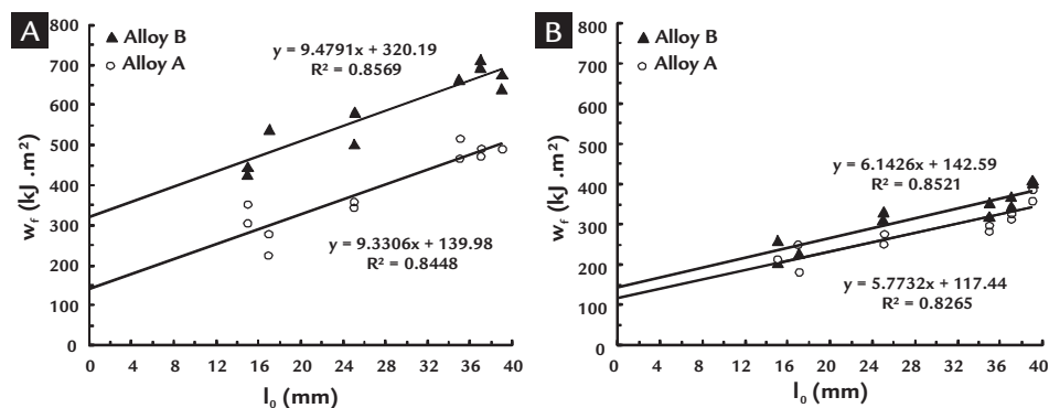
Figure 4 Variation of the specific work of fracture versus ligament length for separation of the essential work of fracture. A) T=1050°C. B) T=1200°C.
