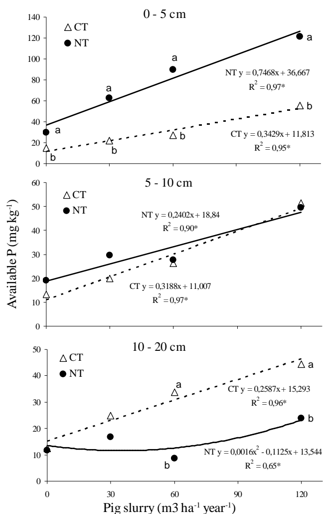
Figure 1. Available phosphorus as affected by the application of increased quantities of pig slurry under conventional or no tillage
