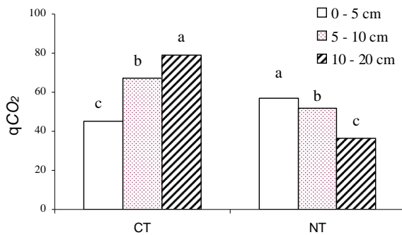
Figure 5. The metabolic quotient ( qCO_2 ) under different depths and soil tillage systems
