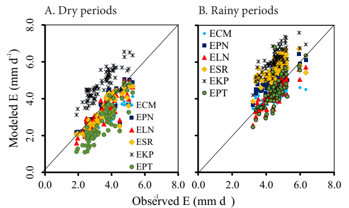
Figure 2. Comparison between E_{20} and evaporation estimated by the models for: (A) dry periods; (B) rainy periods; the index c for each method is indicated
