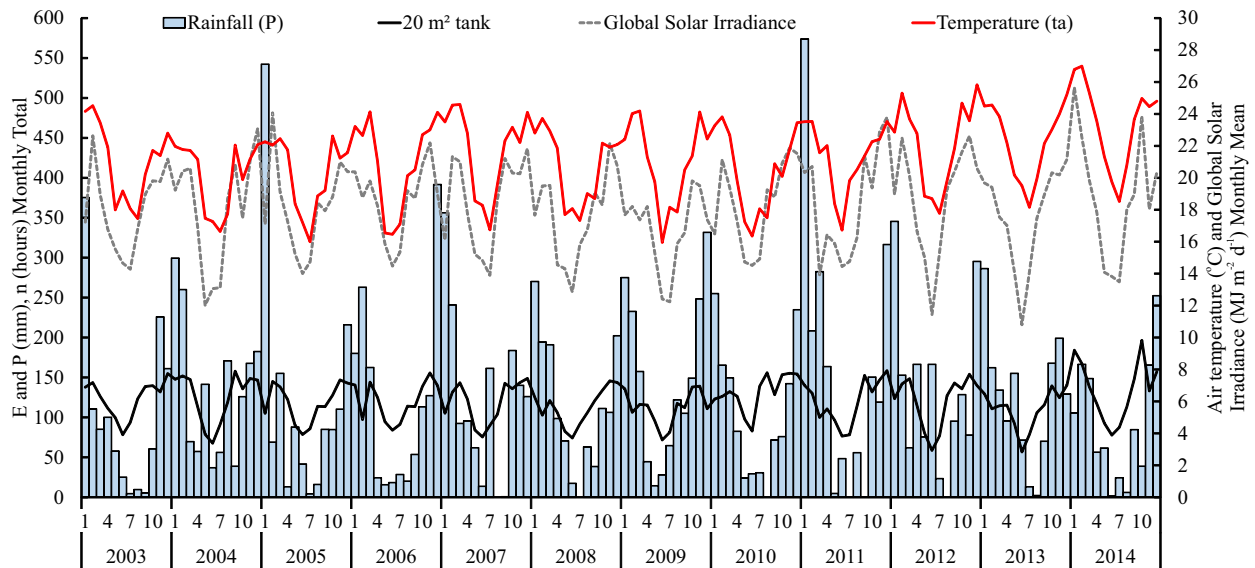
Mean R_s observed in the months is shown in \text{MJ m}^{-2} \text{d}^{-1} . Mean air temperature ( ^{\circ}\text{C} ) is also indicated
