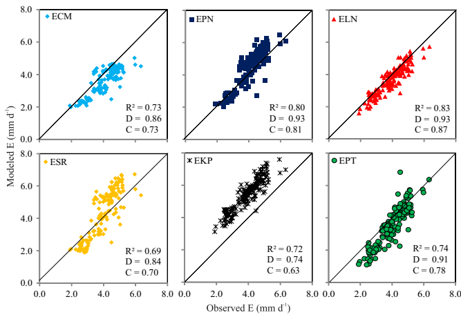
The coefficients of correlation ( R^2 ); agreement (D) and performance (C) are also described Figure 3. Comparison between E_{20} and estimates for the entire period of 2003-2014
