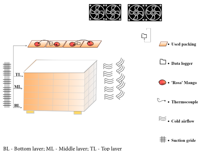
Figure 1. Diagram of the fast-cooling room with a pallet and thermal sensors connected to fruits in each layer
