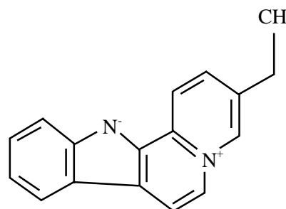
Flavopereirine
