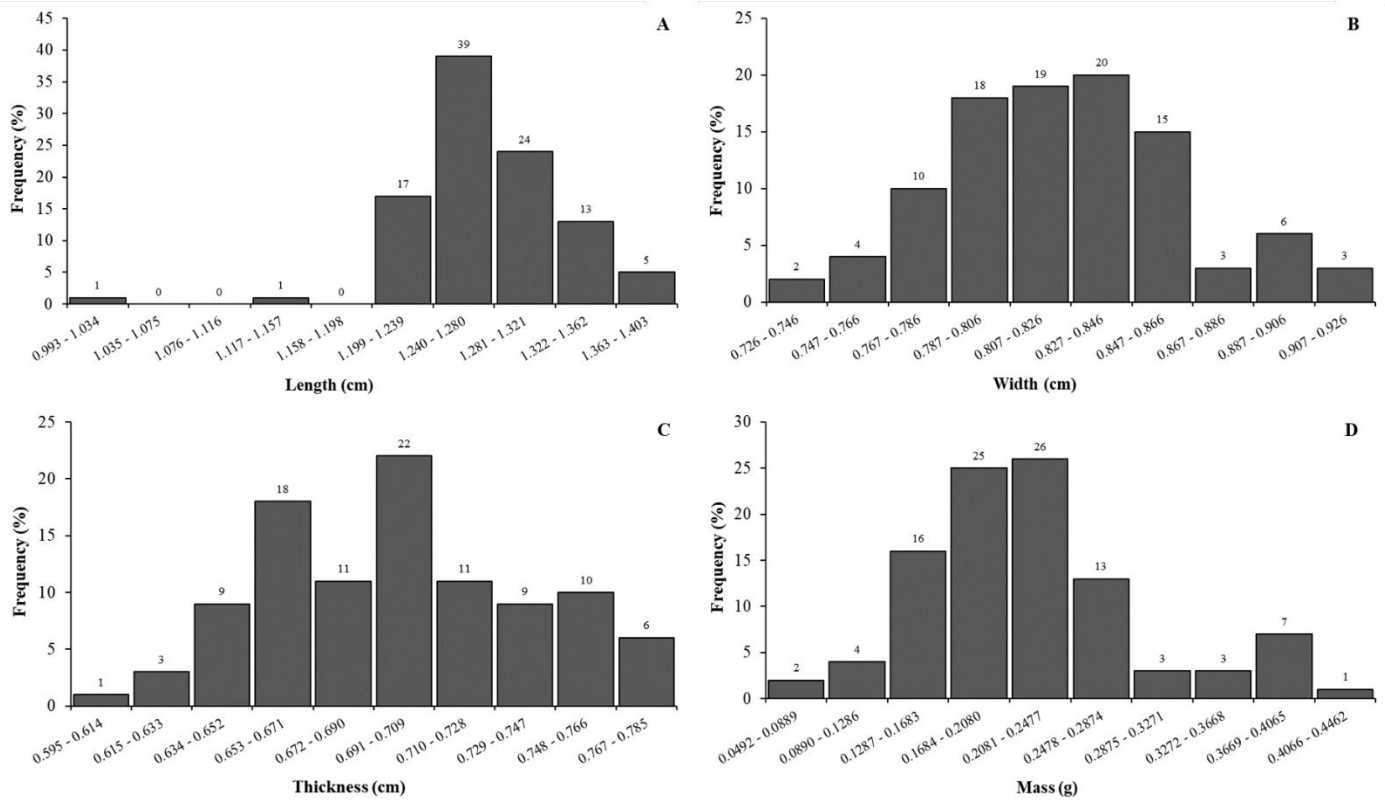
Figure 2. Percentage of frequency of length (A), width (B), thickness (C), and mass (D) of J. mollissima seeds.
