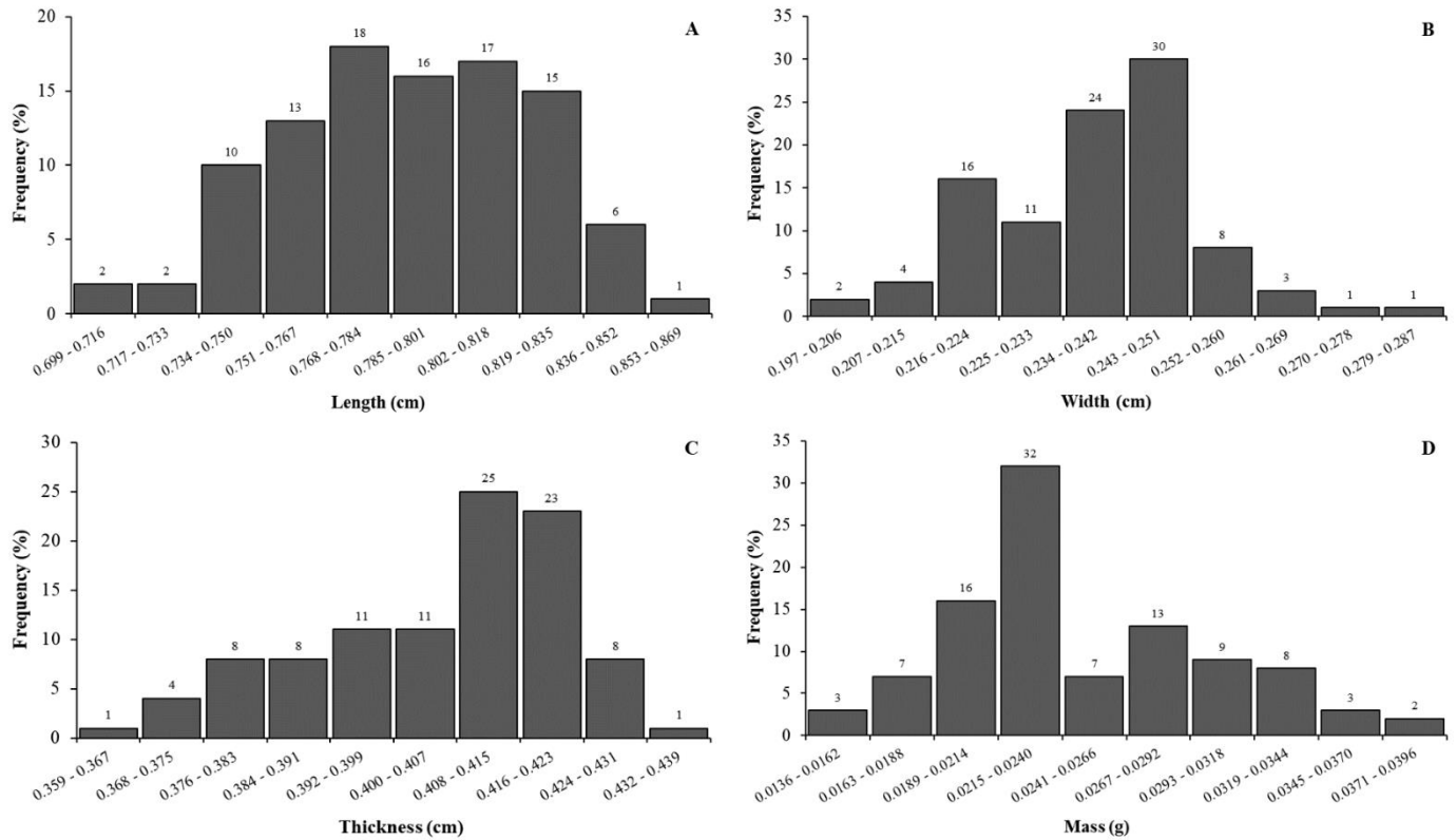
Figure 3. Percentage of frequency of length (A), width (B), thickness (C), and mass (D) of C. urens seeds.
