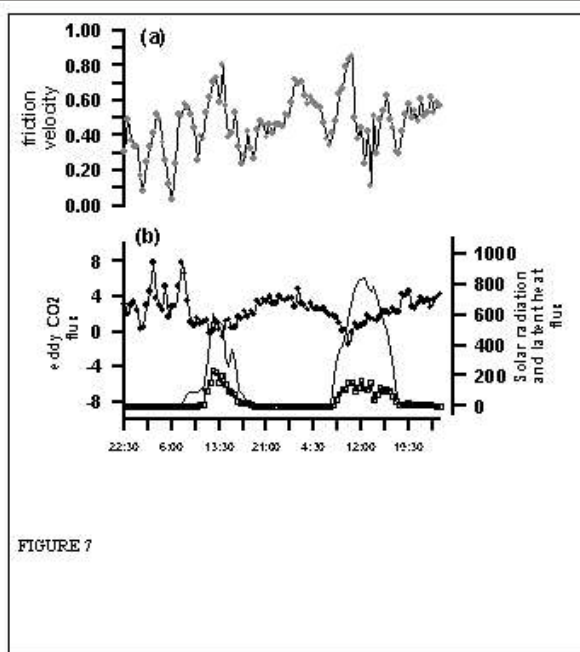
Figure 7. Diel course (Local Time) of 30-minute (a) (left axis) friction velocity measured at 21 m, in \text{ms}^{-1} (black dots); (b) (left axis) eddy \text{CO}_2 flux, in \text{mol CO}_2 \text{ m}^{-2} \text{ s}^{-1} (black dots); (right axis) solar radiation (thin line) and latent heat flux (square dots), in \text{W m}^{-2} . Data are shown for the days 8 and 9 October 2001.
