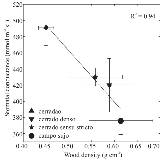
Figure 6. Stomatal conductance in relation to weighted average wood density for sites differing in tree density (cerradão, cerrado denso, cerrado sensu stricto and campo sujo). Each point represents the mean values \pm SE of 10 to 16 tree species per site. Line is the linear regression fitted to the data: y = 780 - 634x ; P < 0.05 .
