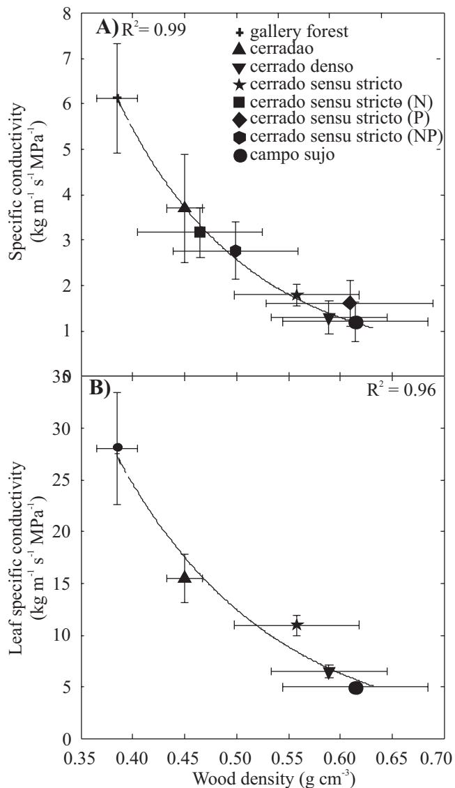
Figure 7. Specific hydraulic conductivity (a) and leaf specific hydraulic conductivity (b) in relation to weighted average wood density for sites differing in tree density (cerradão, cerrado denso, cerrado sensu stricto, campo sujo, gallery forest and cerrado sensu stricto sites subjected to long term fertilizations with N, P and N+P). Each point represents the mean value \pm SE of 10 to 16 species per site. For the gallery forest site only five dominant species were used. The lines are the exponential decaying functions fitted to the data: (a) y = 1.06 + 222 \exp(-11x) ; P < 0.05 ; (b) y = 372 \exp(-6.8x) ; P < 0.001 .
