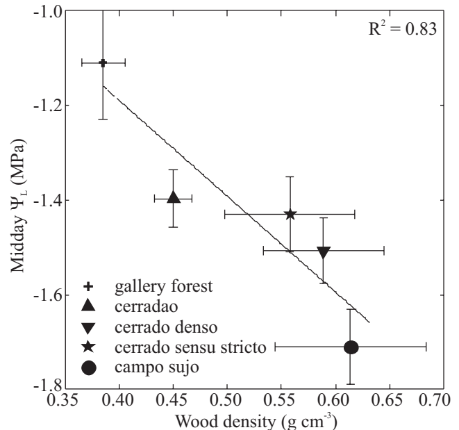
Figure 8. Midday leaf water potential in relation to weighted average wood density for sites differing in tree density (cerradão, cerrado denso, cerrado sensu stricto, campo sujo and gallery forest). Each point represents the mean value \pm SE of 10 to 16 species per site. For the gallery forest site only five dominant species were used. The line is the linear regression fitted to the data: y = -0.38 - 2.02x ; P < 0.05 .
