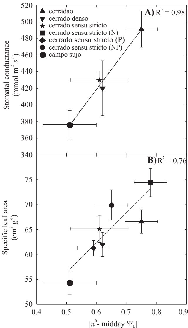
Figure 5. Mean stomatal conductance (a) and mean specific leaf area (b) in relation to mean safety margin for turgor loss ( \pi^0 -midday \Psi_l ) for sites differing in tree density (cerradão, cerrado denso, cerrado sensu stricto and campo sujo) and cerrado sensu stricto sites subjected to long term fertilization with N, P and N+P. Each point represents the mean values \pm SE of 10 to 16 tree species per site. Lines are the linear regressions fitted to the data: (a) y = 130 + 481x ; P < 0.001 ; (b) y = 26 + 60x ; P < 0.05 .
