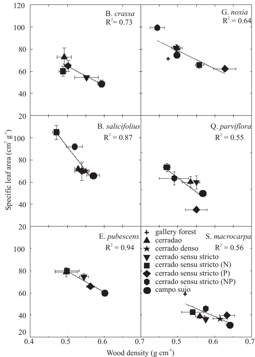
Figure 2. Specific leaf area in relation to wood density for six species growing in sites differing in tree density (cerradão, cerrado denso, cerrado sensu stricto, campo sujo sites and gallery forest) and cerrado sensu stricto sites subjected to long-term fertilization with N, P and N+P. The following species with wide distribution along the gradient were included in the figure: Byrsonima crassa , Blepharocalyx salicifolius , Eriotheca pubescens , Guapira noxia ( Guapira aereolata in the gallery forest site), Qualea parviflora and Schefflera macrocarpa ( Schefflera morototoni in the gallery forest site). Each symbol represents the mean value ± SE of 3 to 6 individuals per species and per site.
