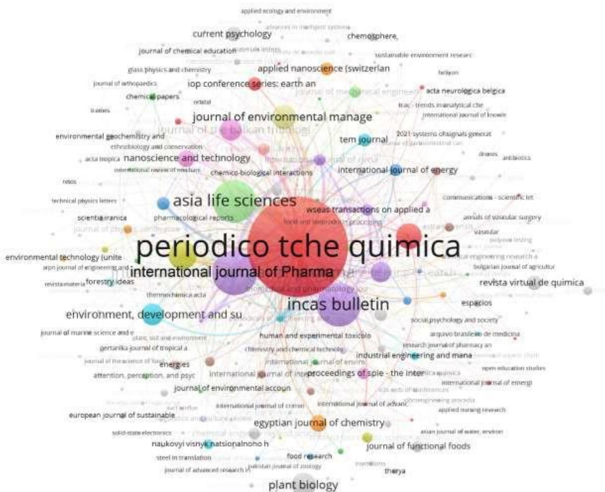
Figure 1. Citation Network
