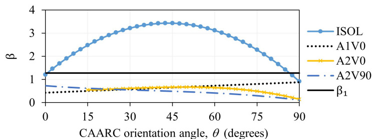
Figure 8. Reliability index \beta for acceleration, x-direction – limit criterion of 4.8 \text{ cm/s}^2 .
